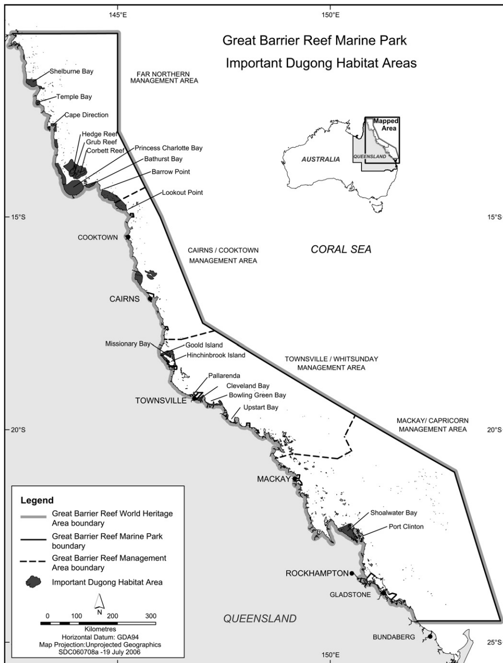
Fig. 1. Important dugong habitats in the Great Barrier Reef World Heritage identified for the Representative Areas Program.
