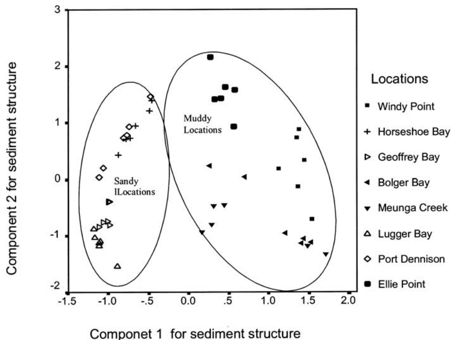
Figure 2. Intertidal areas (locations) categorized by sediment types (muddy or sandy) using Principle Component Analysis.
